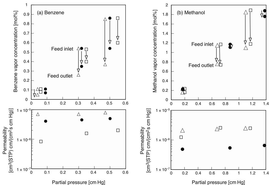
Fig. 2. Removing of VOC vapor in air by liquid membranes: (a) benzene vapor and (b) methanol. \square : TEG liquid membrane ( \delta = 21\text{--}35 \mu\text{m} ), \Delta : TEG-DBE liquid membrane ( \delta = 35\text{--}64 \mu\text{m} ), \bullet : Silicone rubber ( \delta = 72 \mu\text{m} ).
