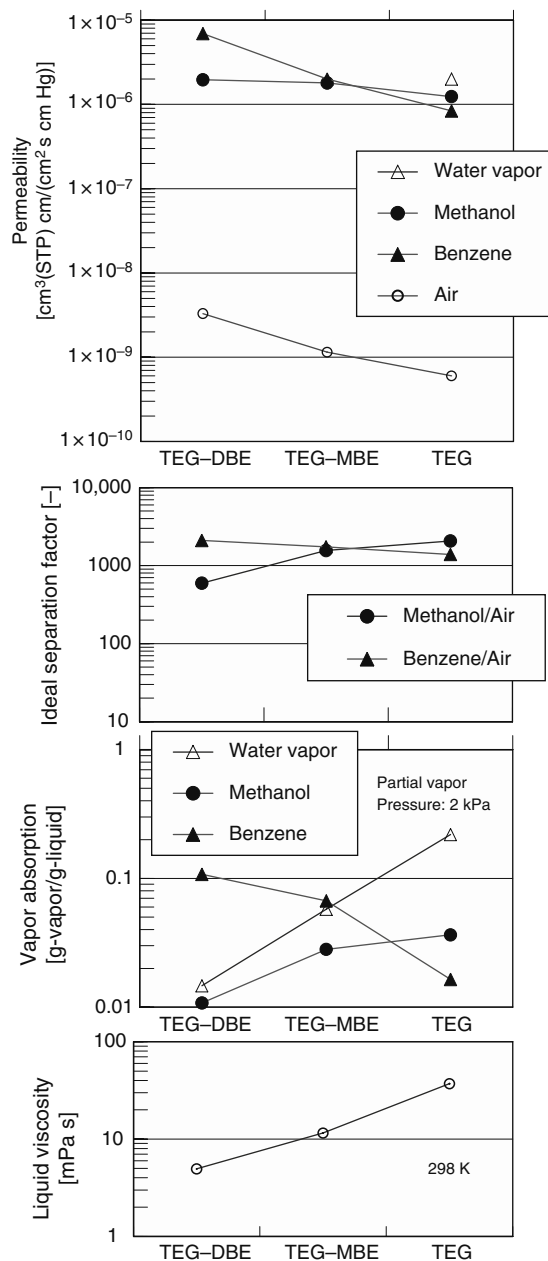
Fig. 5. Relation among vapor permeabilities, separation factors and vapor absorption of benzene, methanol and water vapor for TEG liquid membranes, and liquid viscosity.
