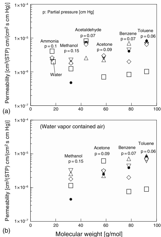
Fig. 3. Permeabilities of VOC vapors through TEG liquid membranes and silicone rubber. □: TEG liquid membrane ( \delta = 21\text{--}53 \mu\text{m} ), \triangle : TEG–DBE liquid membrane ( \delta = 12\text{--}85 \mu\text{m} ), \nabla : TEG–DME liquid membrane, ( \delta = 34\text{--}79 \mu\text{m} ), \diamond : TEG–MBE liquid membrane ( \delta = 23\text{--}35 \mu\text{m} ), ●: silicone rubber ( \delta = 72 \mu\text{m} ).
