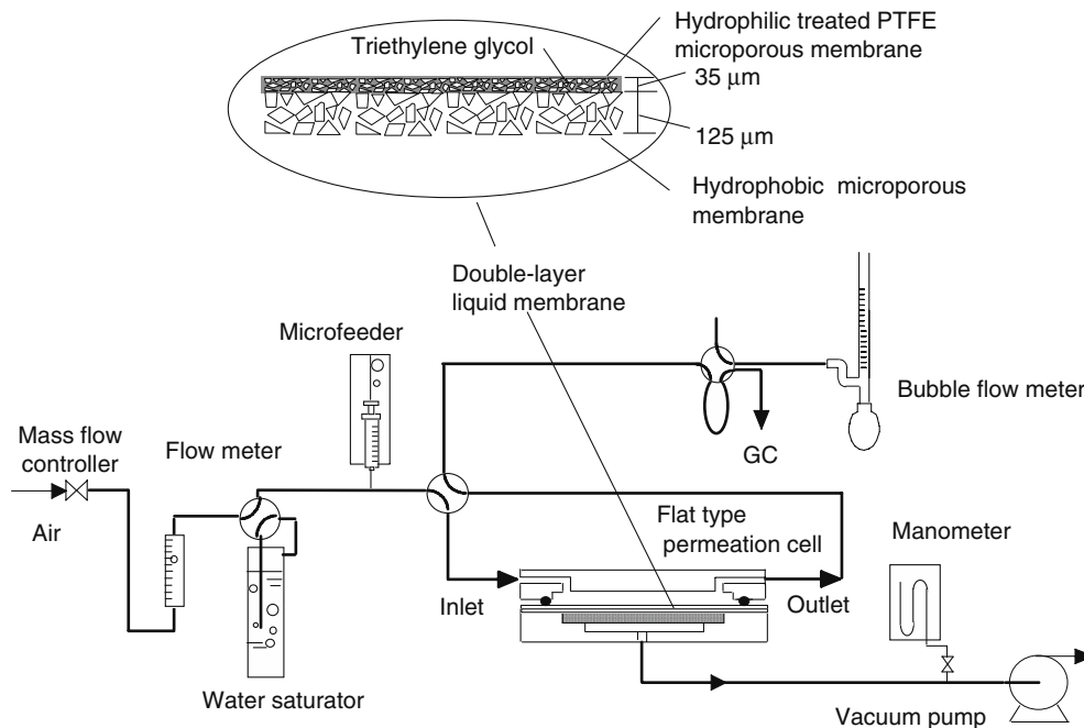
Fig. 1. Experimental setup for vapor permeation through TEG liquid membranes.
