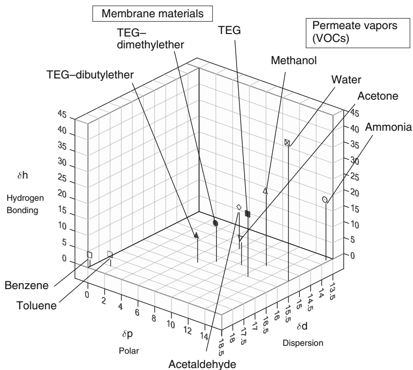
Fig. 4. Hansen solubility parameters of VOCs and the liquid membrane materials.
